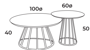
Mesa de centro Coffee Table SET OR43251 - 330P Lacado Lacquered: 308 / 150 Patas Legs: 150
