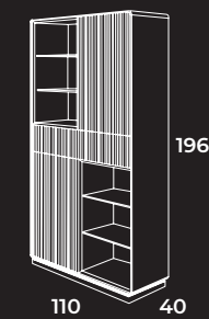
Vitrina Display Unit CU64516 - 700P Lacado Lacquered: 304 / 308
